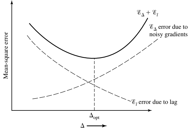
Figure 2.2 Excess mean-square error \mathcal{E}_\Delta and lag error \mathcal{E}_l as a function of the step size \Delta .
