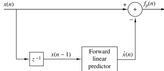
Figure 3.1 Forward linear prediction.
