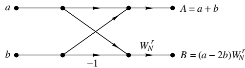
Figure 1.10 Basic butterfly computation in the decimation-in-frequency FFT algorithm.
