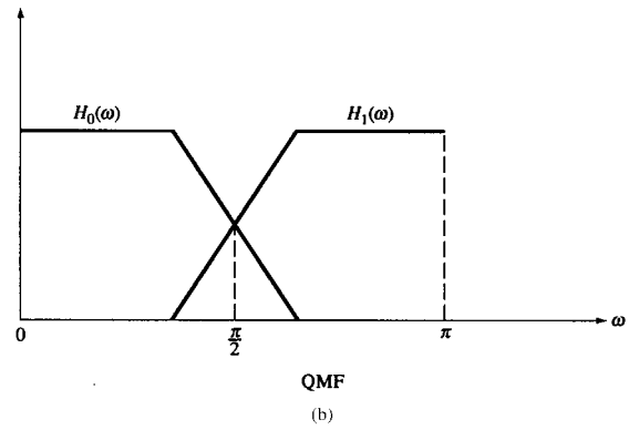
Figure 9.5 Filter characteristics for subband coding.
