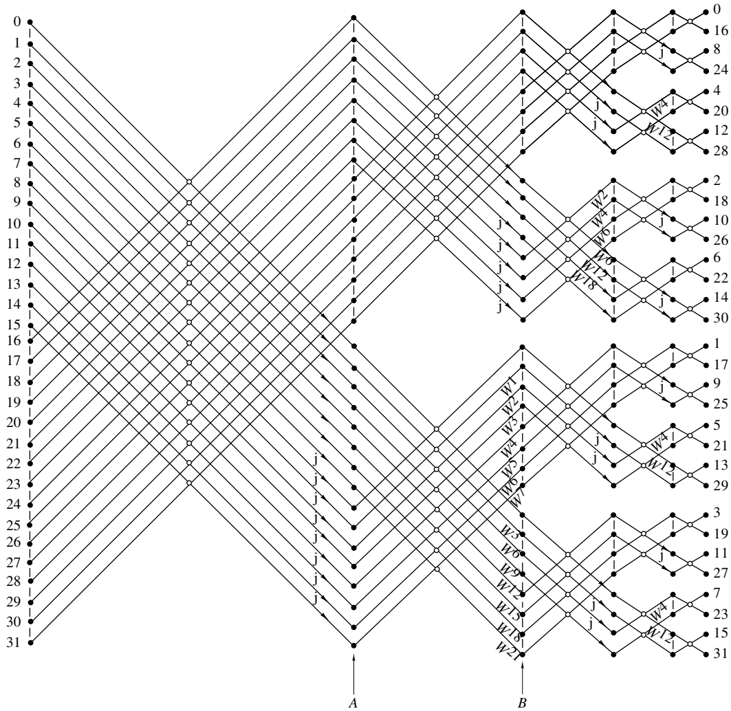
Figure 1.15 Length 32 split-radix FFT algorithms from paper by Duhamel (1986); reprinted with permission from the IEEE.
